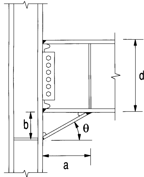
Figure 6.1 Haunch Geometry
